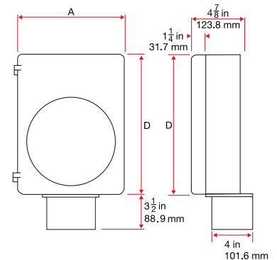
Pedestal Mounted
