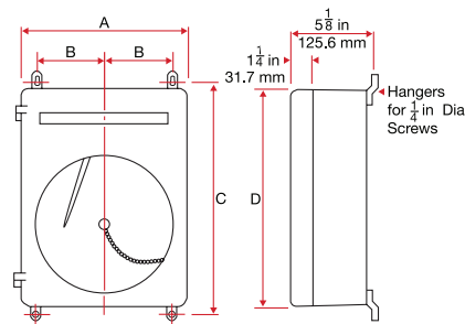
Wall Mounted
