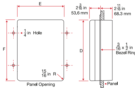
Flush Mounted
