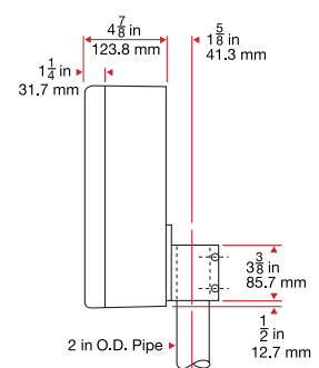
Pedestal Mounted
